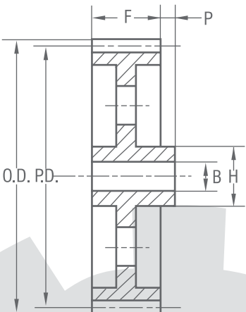
Type B2
