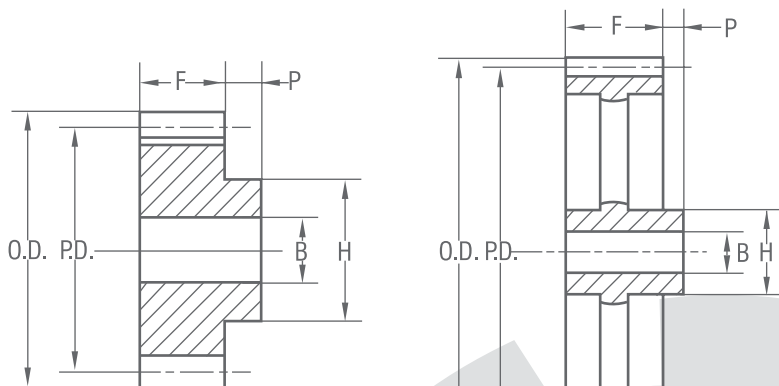
Type B
