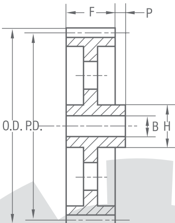
Type B2
