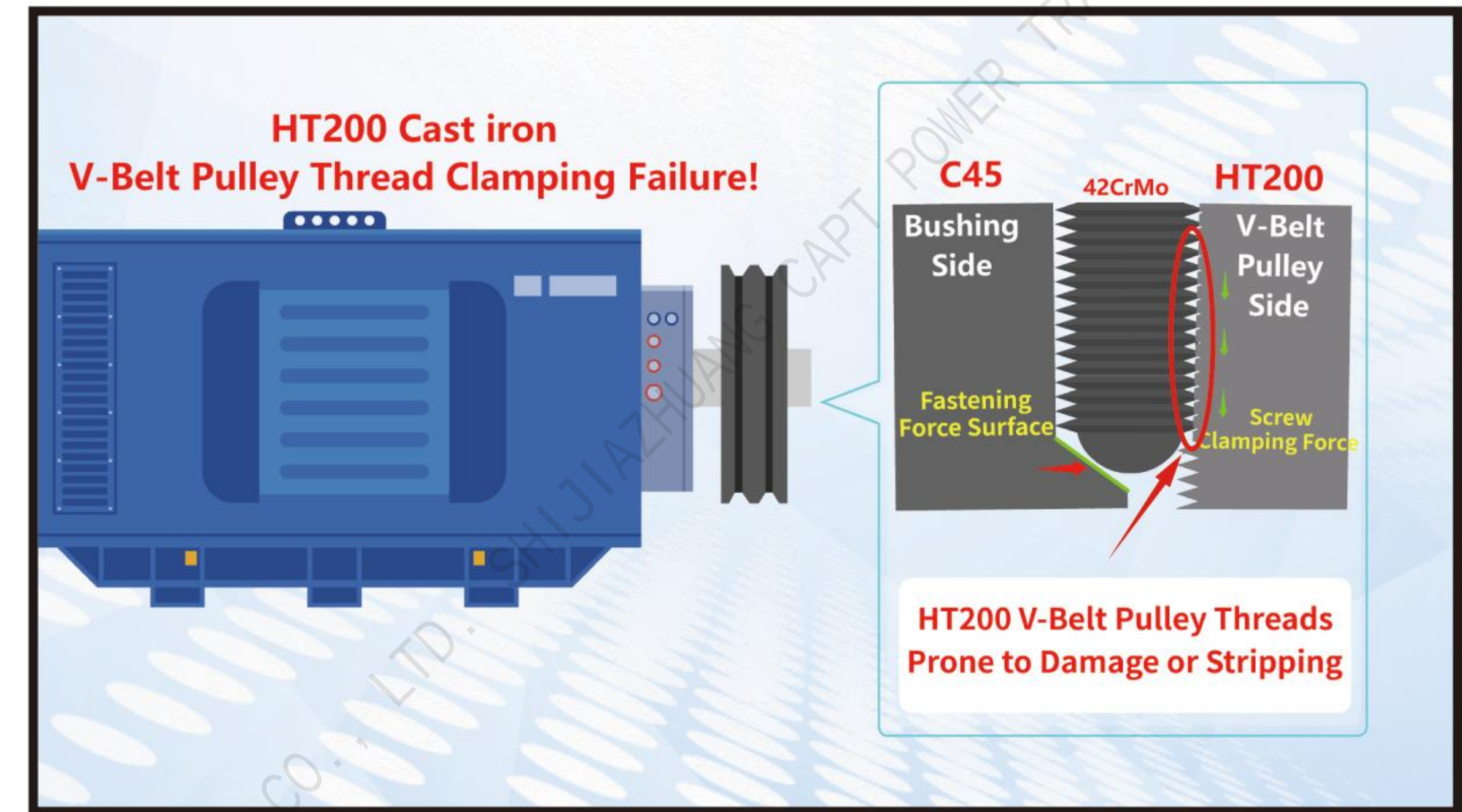
⑭The threads in HT200 cast iron pulleys are easily stripped and damaged.
