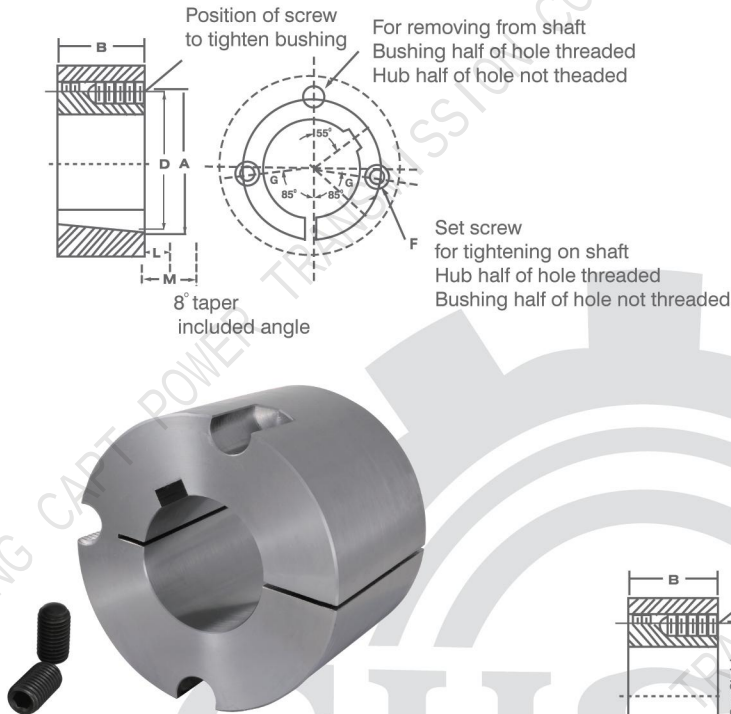
Dimensions for 1008 thru 3030 BTL Taper Bushings
